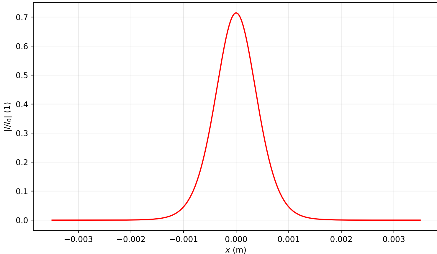
Intensity profile I(x, y = 0, z = 2.388)/I_0 , P_{in}=0.5P_{cr} , artificial time
